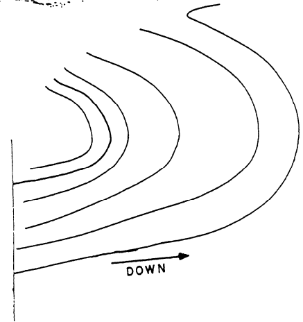
Figure 5-9.—Concave slope.
