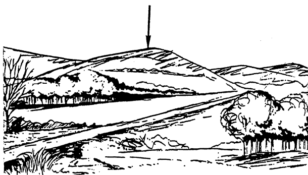
Figure 5-10.—Convex slope.
