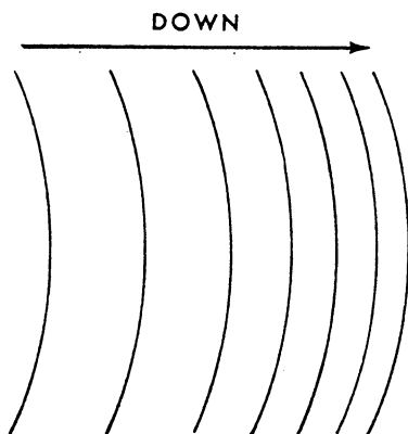
Figure 5-10.—Convex slope.
