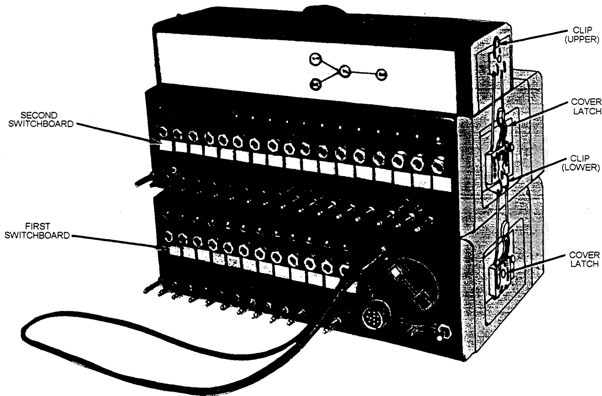
Figure 11-26.—Installation arrangement for two switchboards.
