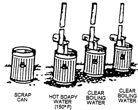
Figure 10-57.—Immersion heaters for mess kit washing setup.
