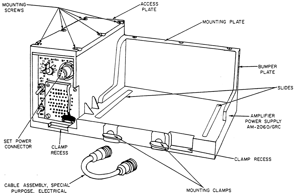
Figure 11-4B.—Amplifier AM-7060 for Radio Set AN/GRC-160.
