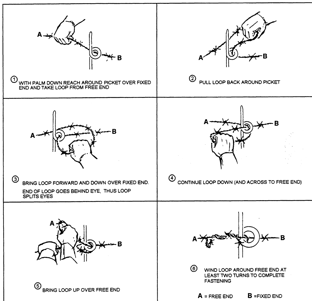
Figure 8-15.—Intermediate-eye tie.
