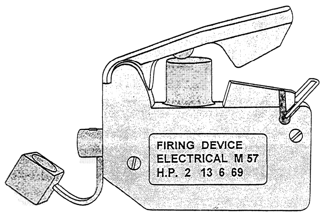
Figure 12-16.—The M57 firing device.
