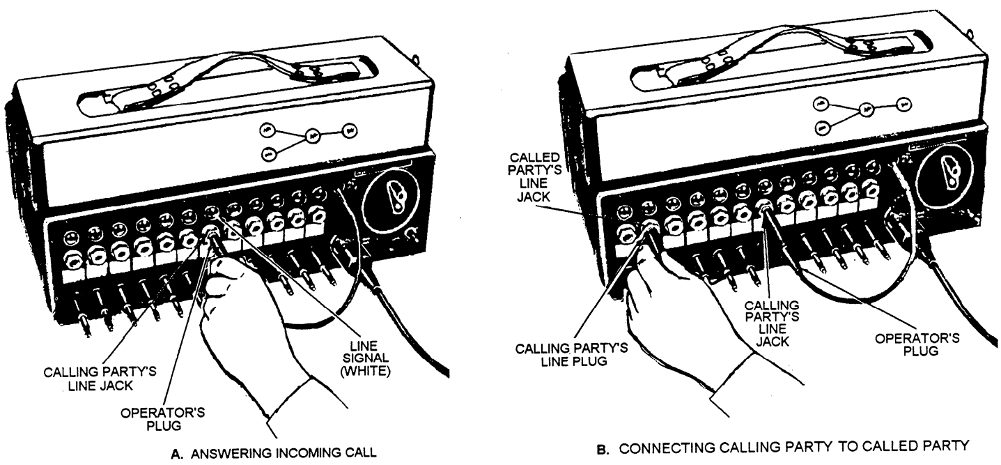
Figure 11-25A and B.—Steps required to connect local calls through the SB-22/PT switchboard.
