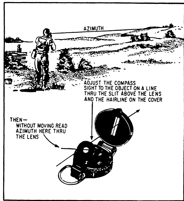
Figure 5-28.—A method of determining the azimuth of a visible object.
