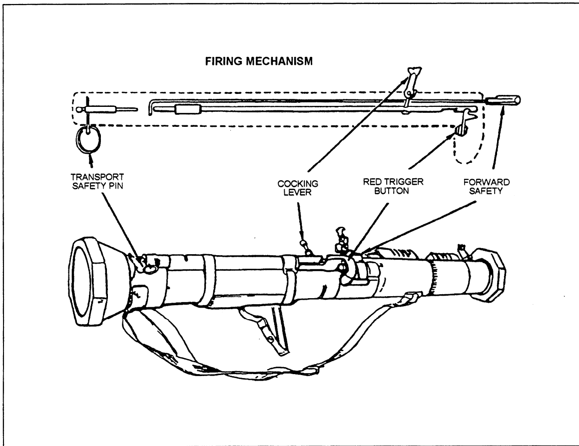
Figure 14-28.—Firing mechanism.
