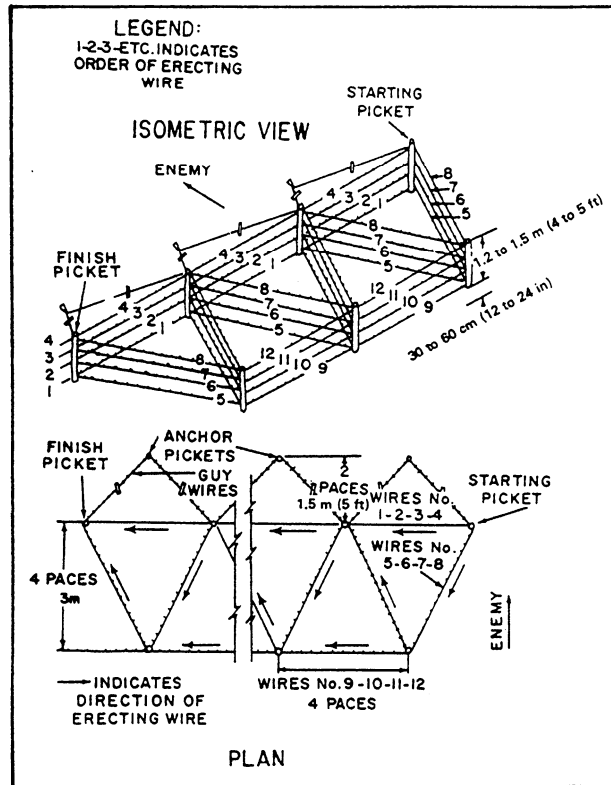
Figure 8-20.—High-wire entanglement.
