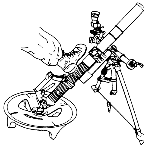
Figure 14-21.—Misfire procedure: Dislodging the round.
