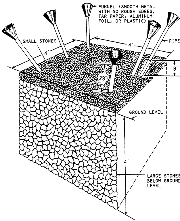
Figure 10-56.—Urinal pipes and soakage pit.
