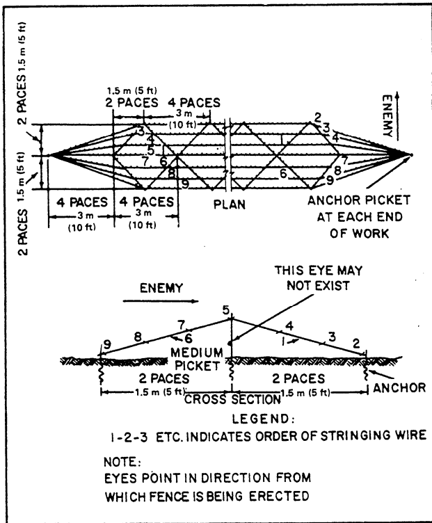
Figure 8-29.—Low-wire fence.
