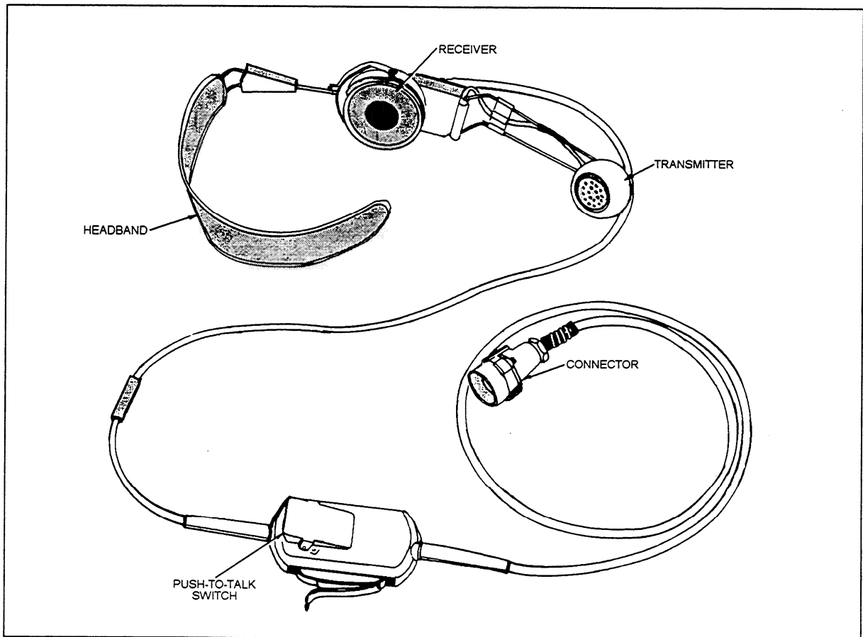
Figure 11-21.—Handset-headset, H81A/U.
