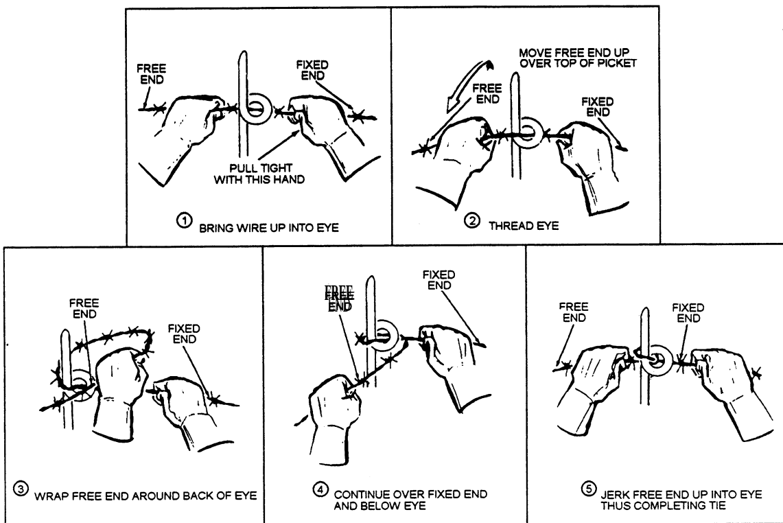
Figure 8-14.—Top-eye tie.
