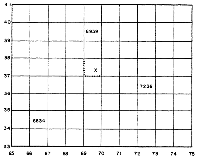
Figure 5-4.—Grid system.
