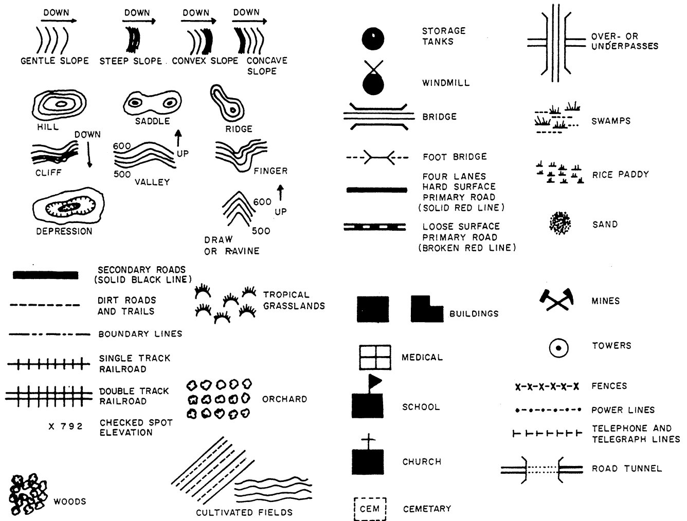
Figure 5-22.—Topographic symbols.
