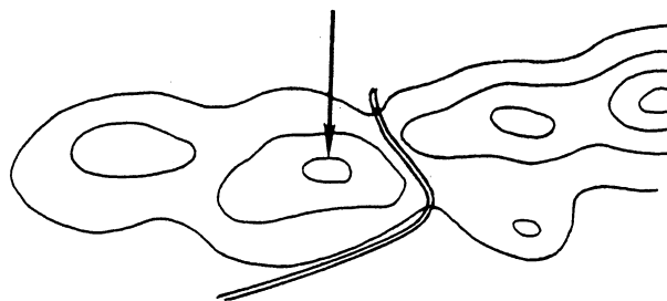
Figure 5-11.—Hill.
