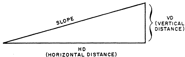
Figure 5-18.—Slope diagram.
