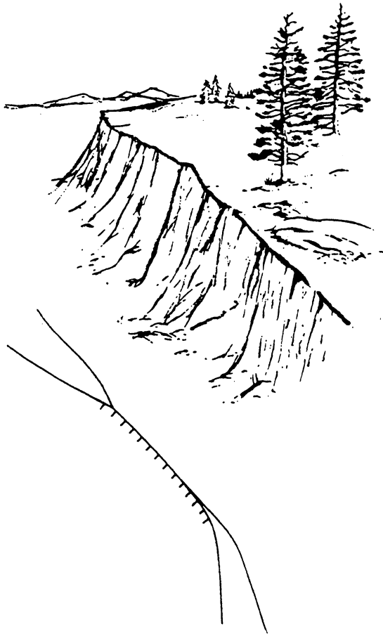
Figure 5-15.—Cliff.
