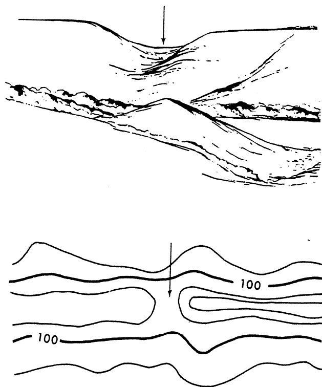
Figure 5-14.—Saddle.
