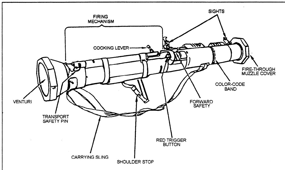
Figure 14-26.—Launcher components.
