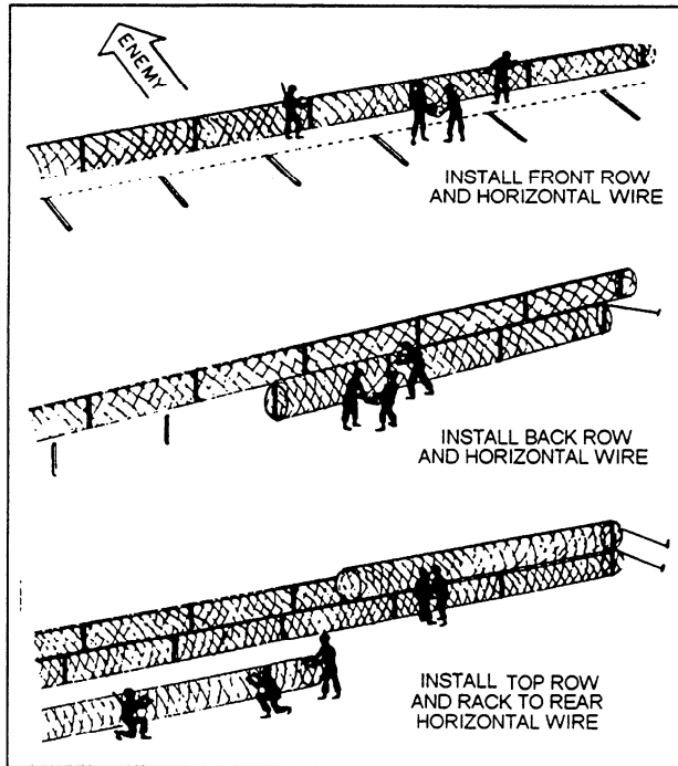
Figure 8-27.—Installing concertina.
