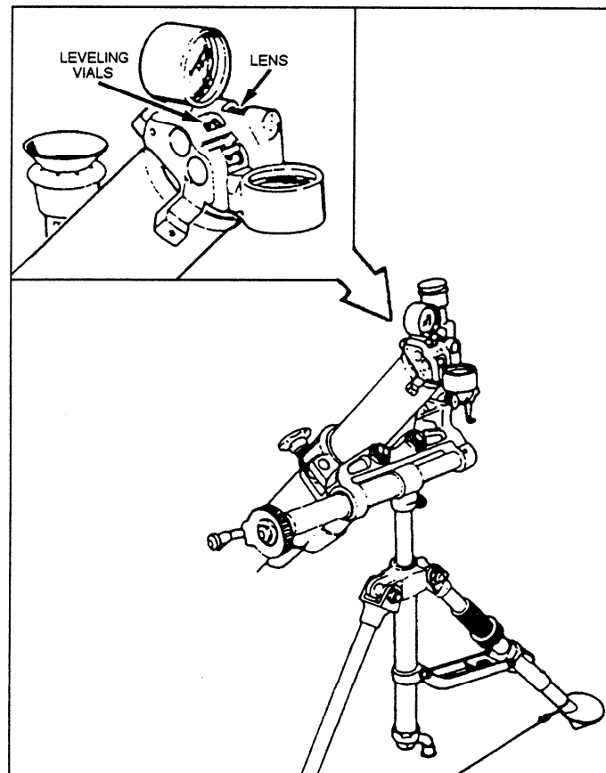
Figure 14-6.—Boresight (M115).
