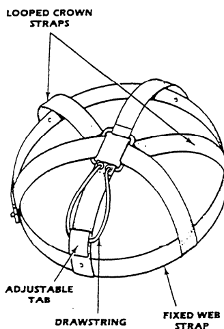
Figure 2-31.—Suspension band.
