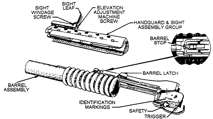
Figure 13-2.—The 40-mm grenade launcher M203, controls, and their identifications.
