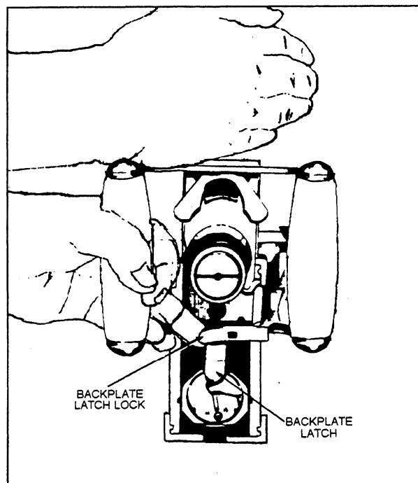
Figure 13-46.—Replacing the backplate assembly.
