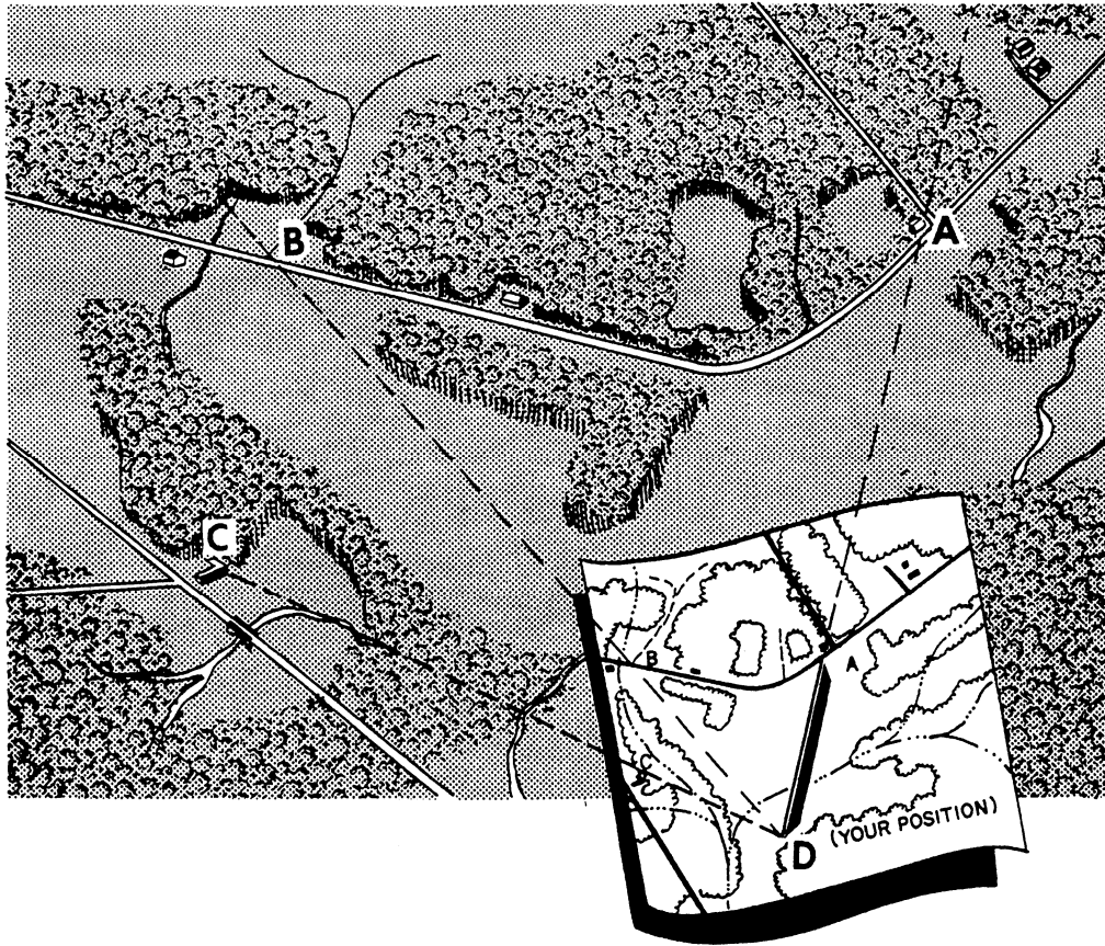
Figure 5-38.—Resection.
