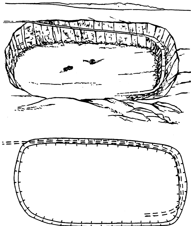
Figure 5-17.—Depression.
