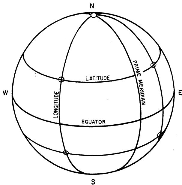
Figure 5-3.—Position location.
