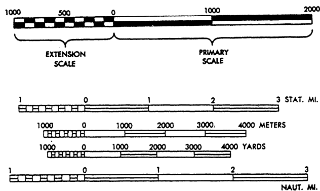
Figure 5-19.—Graphic scale.
