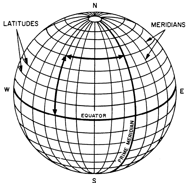
Figure 5-2.—Reference lines.
