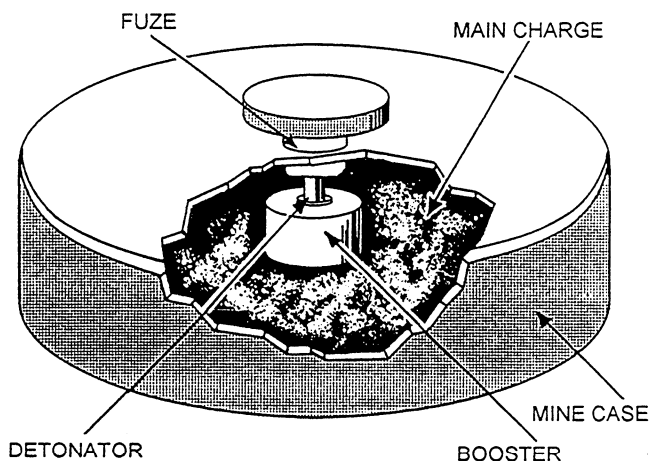
Figure 12-12.—Typical pressure type of land mine mechanism.
