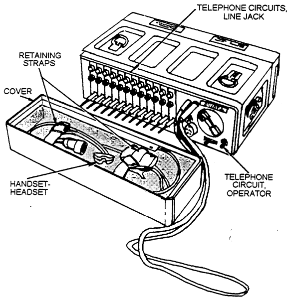
Figure 11-17.—Manual SB-22/PT telephone switchboard.
