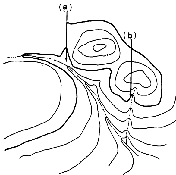
Figure 5-12.—(a) Valley; (b) Draw.
