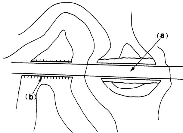
Figure 5-16.—(a) Cut; (b) Fill.
