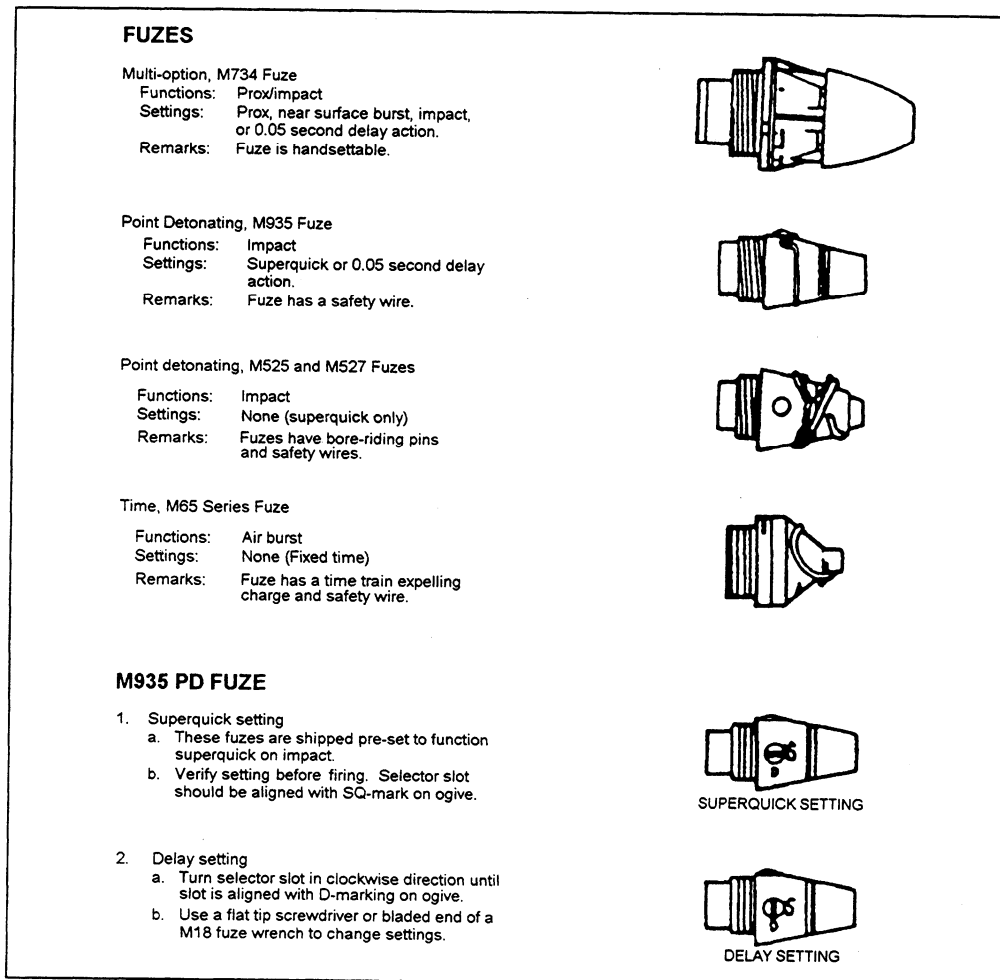
Figure 14-11.—Fuzes.
