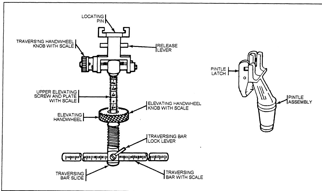
Figure 13-12.—Traversing and elevating mechanism, pintle, and platform group.
