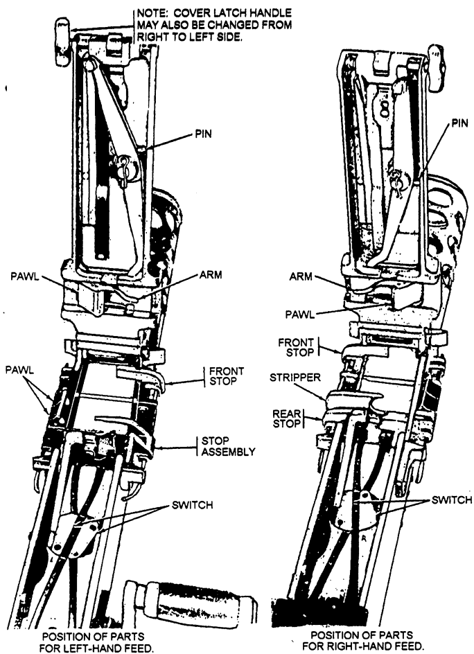
Figure 13-47.—Feeding mechanism parts of the receiver setup for left-hand and right-hand feeding.
