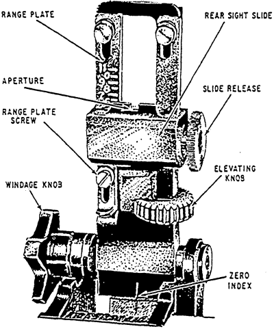
Figure 13-7.—The rear sight.
