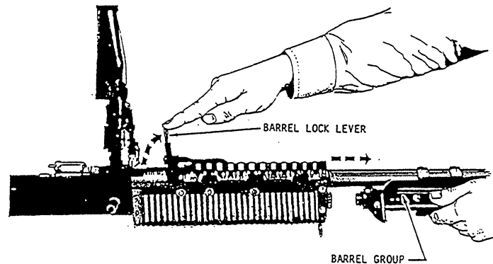
Figure 13-24.—Removing the barrel group.
