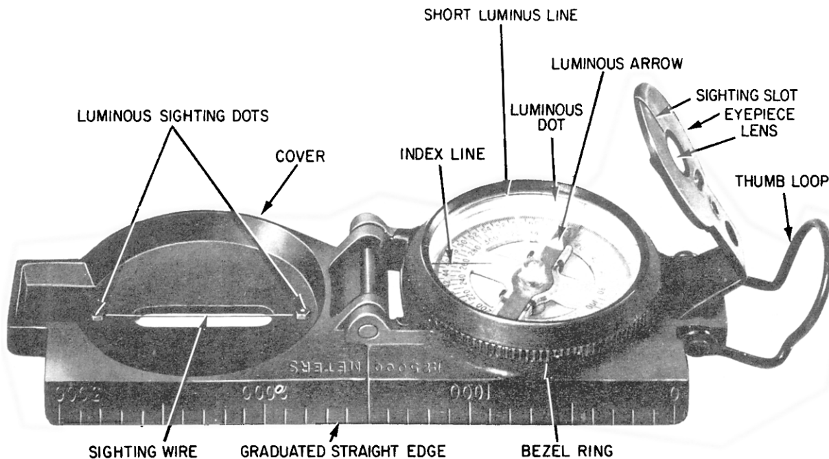
Figure 5-26.—Lensatic compass.
