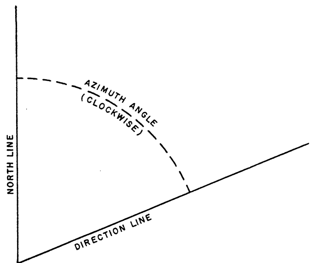
Figure 5-29.—Azimuth angle.
