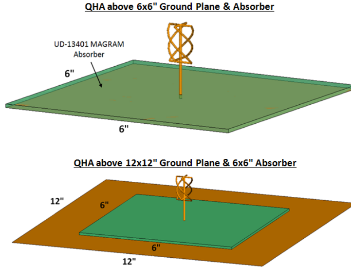
Fig. 8 FEKO models of self-phased quadrifilar helix antenna (QHA) over 6 \times 6 " ground plane with absorber and 12 \times 12 " ground plane with 6 \times 6 " absorber
